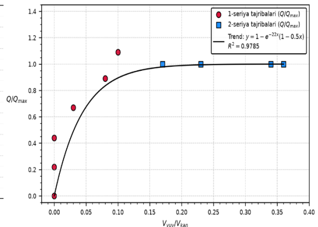
1.2-rasm. Bog‘langan grunt yuvilish hajmining suv sarfiga bog‘liq holda
