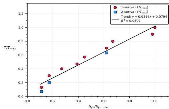
1.7-rasm. Bog‘langan grunt yuvilish chuqurligining vaqtga bog‘liq ravishda
