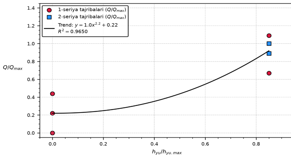
1.3-rasm. Bog'langan grunt yuvilish chuqurligining suv sarfiga bog'liq ravishda
