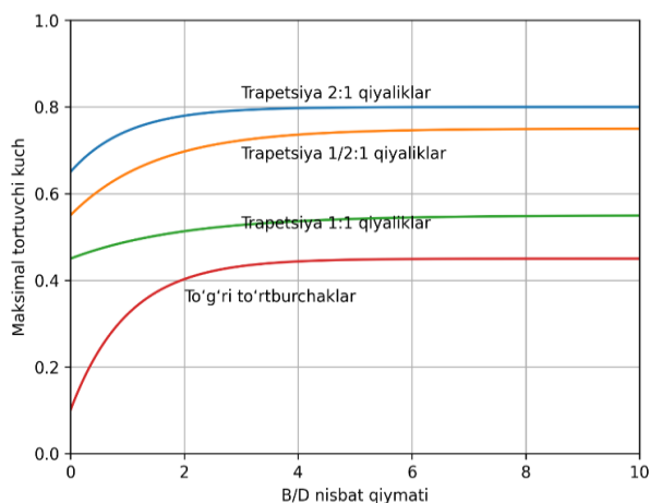
3-rasm. Yon tomon qiyalik uchun.
