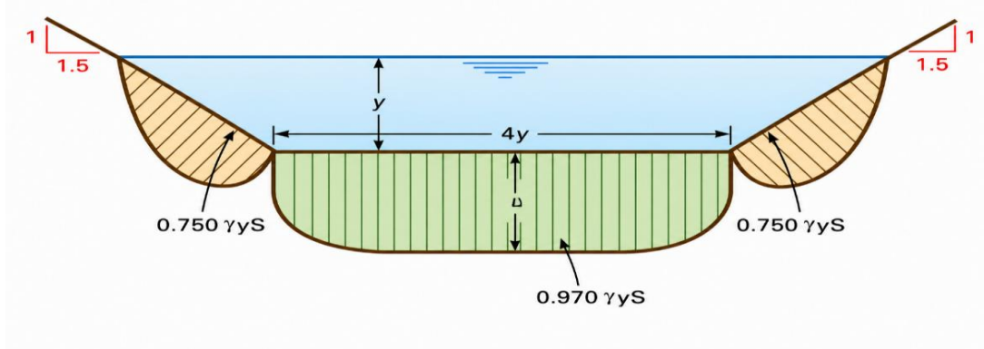
5-rasm. Siljituvchi kuchning taqsimlanishi.
