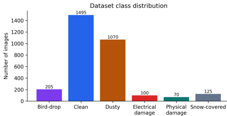
Fig. 2. Class distribution in the PV panel image dataset.
