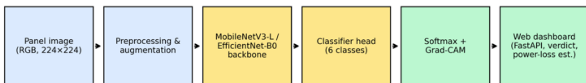
Fig. 1. Overall architecture of the proposed PV soiling and fault detection system.
