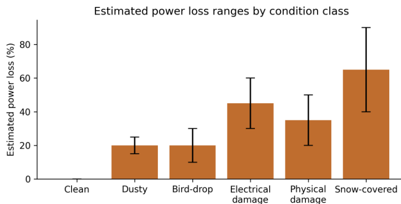
Fig. 6. Estimated power loss ranges by predicted condition class.
