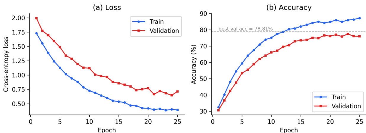
Fig. 3. Training and validation (a) loss and (b) accuracy of the MobileNetV3-Large model. Source: author's calculations.
