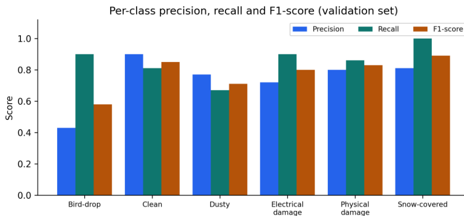
Fig. 5. Per-class precision, recall and F1-score on the validation set.
