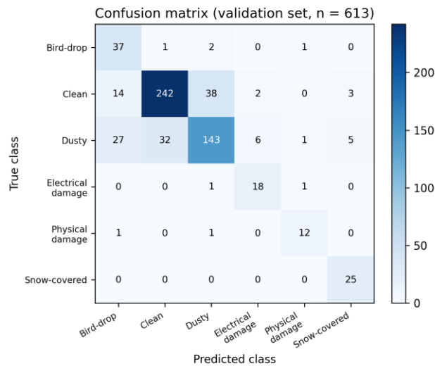
Fig. 4. Confusion matrix on the validation set (n = 613).
